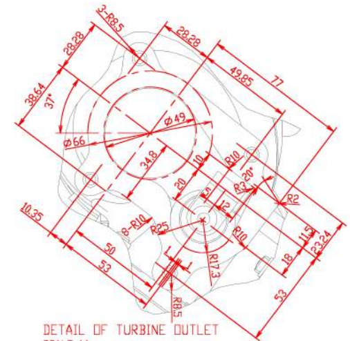
DETAIL OF TURBINE OUTLET
